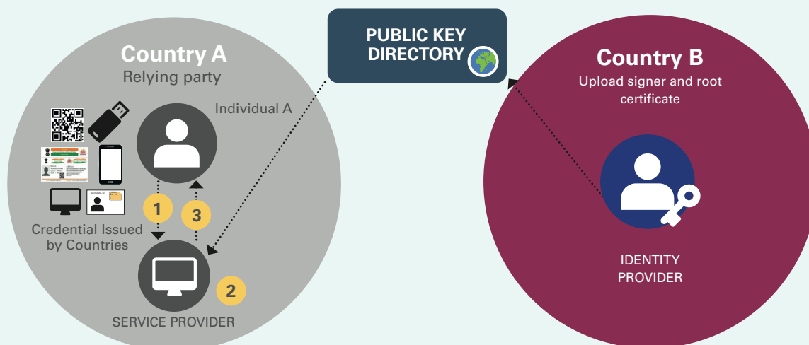
FIGURE 4 – OVERVIEW OF OPTION 3 - DIGITALLY SIGNED CREDENTIALS
