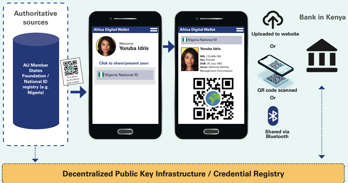
FIGURE 2 – OVERVIEW OF OPTION 1 - PERSONAL DIGITAL WALLETS
